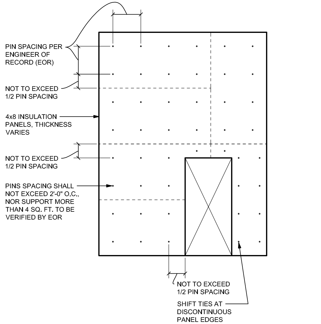
A TYPICAL INSULATION PANEL LAYOUT P100 P100 1/4" = 1'-0"
